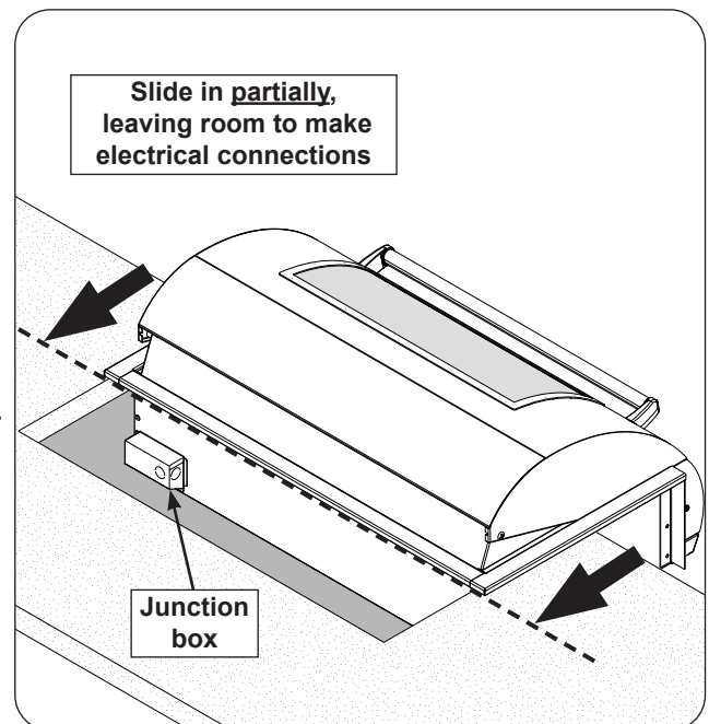
Fig. 22-2 Position unit for wiring
