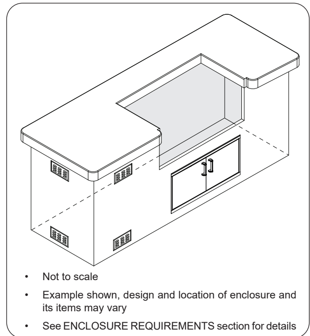
Fig. 22-1 Enclosure construction overview
