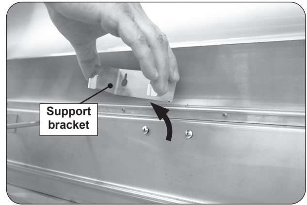
Fig. 24-1 Remove element support bracket
