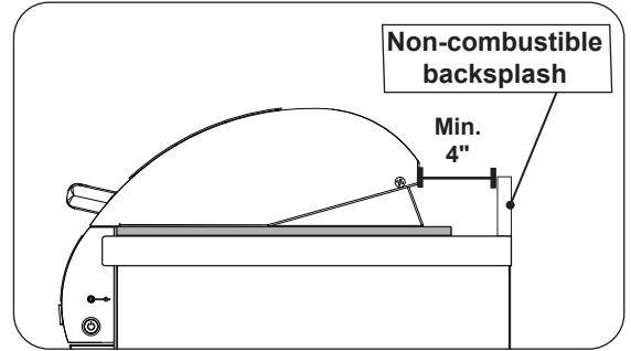
Fig. 13-2 Backsplash clearance
