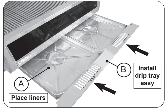
Fig. 26-1 Install drip tray
