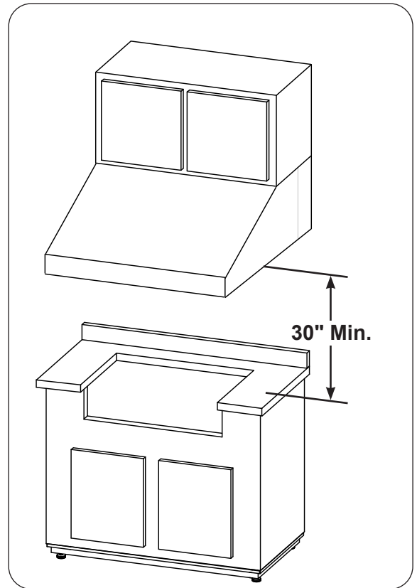
Fig. 12-1 Overhead requirements
